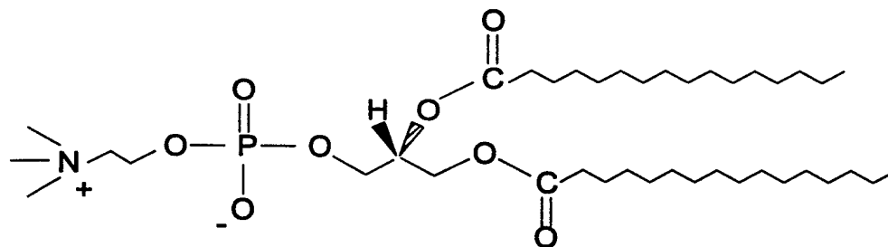
1, 2-Dipalmitoyl-s n-Glycero-3-Phosphocholine (DPPC)
